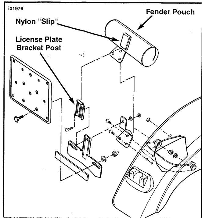
Figure 1. Nylon "Slip" and License Plate Bracket Post.
