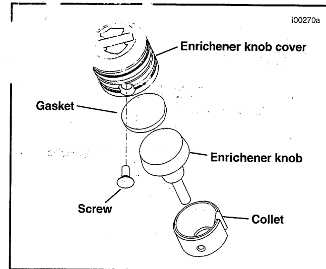
Enrichener Knob Cover Installation
